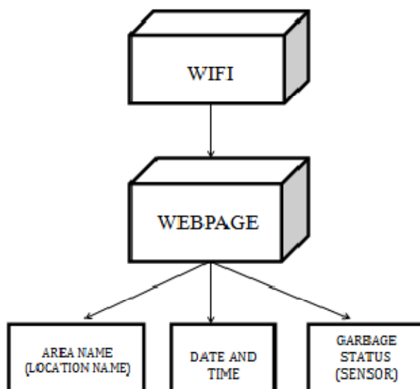
Figure 3.2 Webpage Display
